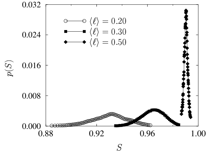
FIG. 2: Distribution of the isolated network size p(S) as a function of S for several values of \langle \ell \rangle . The network is formed by N = 10^4 nodes.
